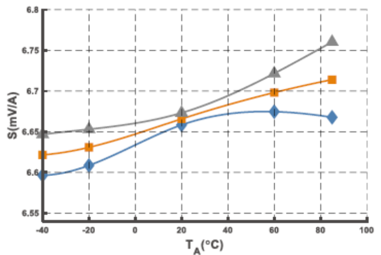
Figure 6. Sensitivity @IPN = 600 A versus ambient temperature
