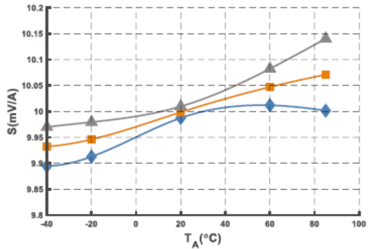
Figure 6. Sensitivity @IPN = 400 A versus ambient temperature
