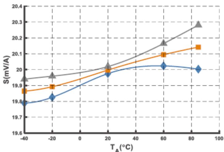
Figure 6. Sensitivity @IPN = 200 A versus ambient temperature
