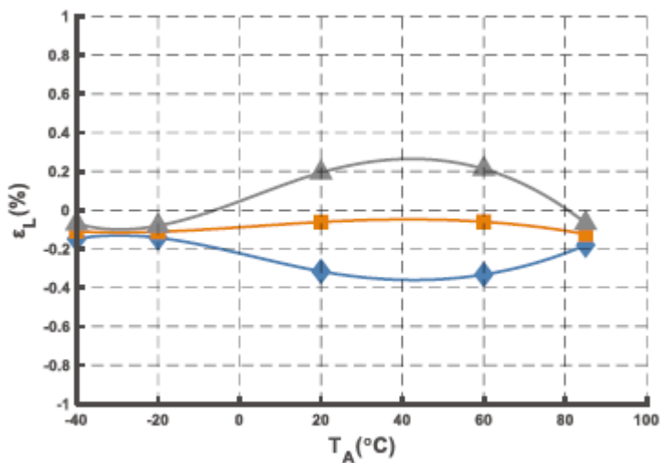
Figure 8. Linearity error versus ambient temperature
