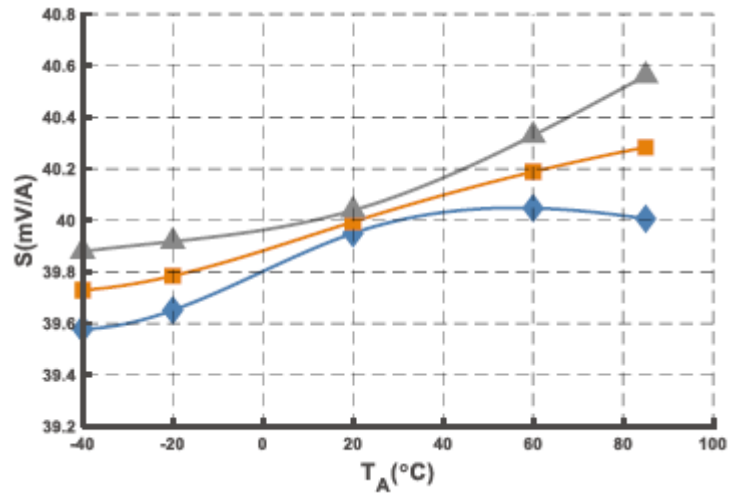
Figure 6. Sensitivity @IPN = 100 A versus ambient temperature
