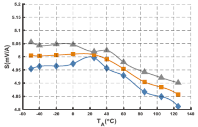
Figure 14. Sensitivity (@ I_{PN} = 800 \text{ A} )
