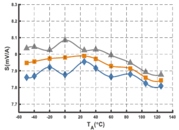
Figure 10. Sensitivity (@ I_{PN} = 500\text{ A} )
