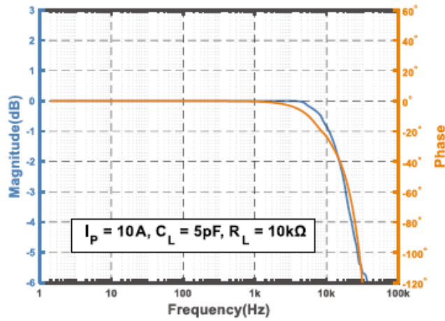
Figure 5. Bode Plot
