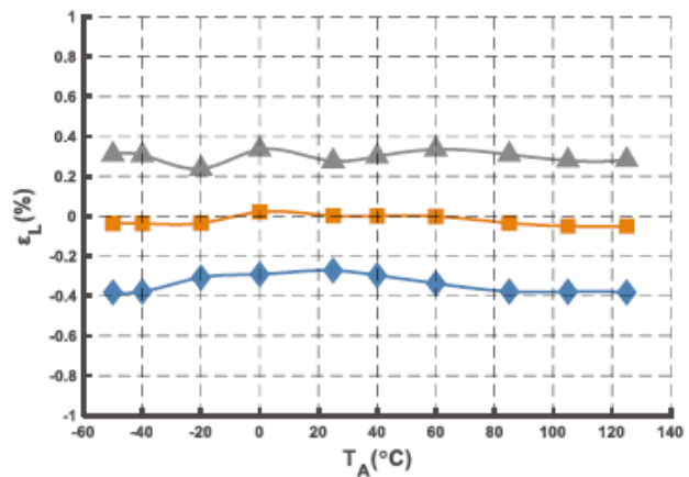
Figure 7. Linearity Error
