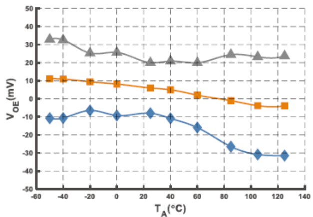
Figure 9. Electric Offset
