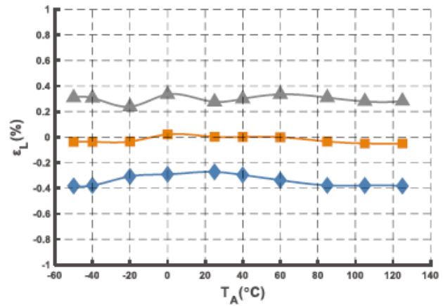
Figure 7. Linearity Error
