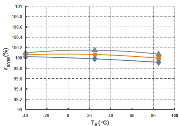
- Symmetry
