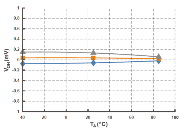
- Hysteresis
