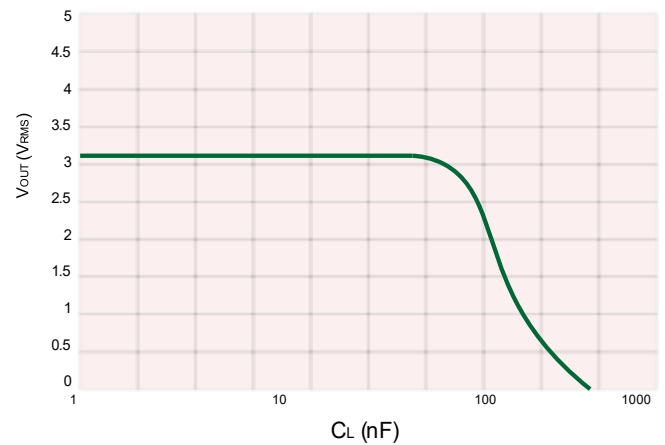
Output Voltage vs Load Capacitance (@ I_P = I_{PN} )
